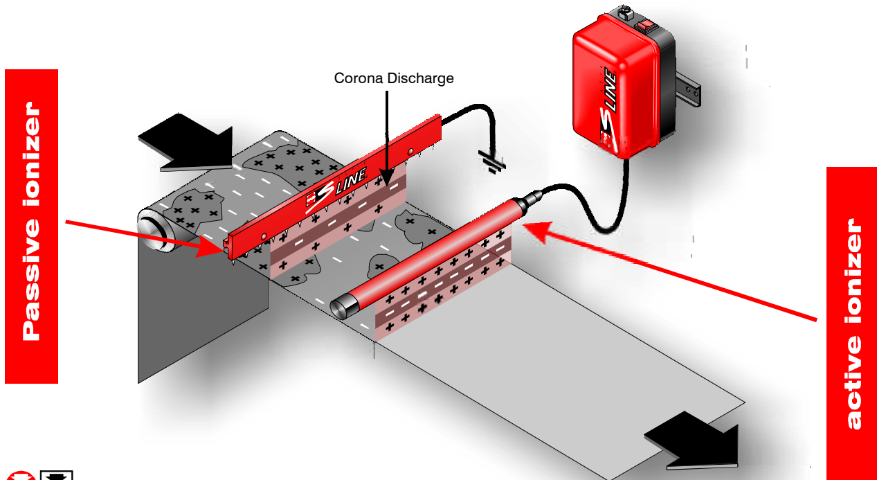
Fig. 3: Passive ionizer
